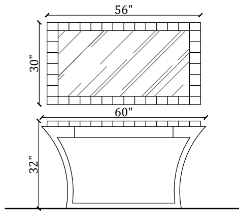
FRONT VIEW WOODEN CONSOLE WITH MIRROR
